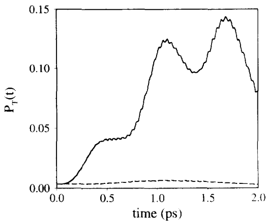
Fig. 3. P_T(t) as a function of time at the resonant frequency \omega_{\text{ac}} = 150 THz (solid line) and out of resonance \omega_{\text{ac}} = 200 THz (dashed line).
