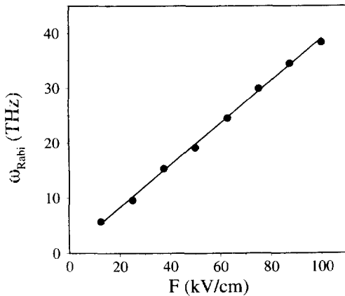
Fig. 2. Rabi frequency as a function of the dc field when the driving frequency is tuned to the resonant frequency \omega_{\text{ac}} = 150 THz
