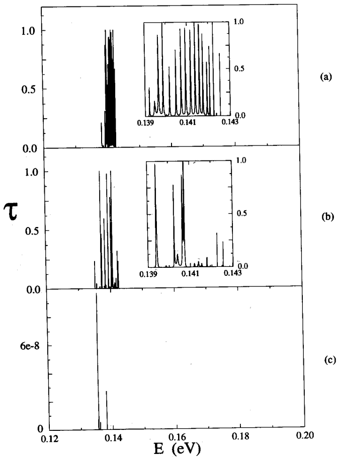
Fig. 3. Transmission coefficient \tau versus energy E for (a) perfect ( W = 0 ) DQWSL, (b) imperfect ( W = 0.05 ) DQWSL, and (c) random ( W = 0 ) QWSL. Every GaAs-Ga 0.65 Al 0.35 As SL consists of N = 200 barriers of b = 32 Å whereas the thicknesses of QW are a = 32 Å and a' = 26 Å. Insets of (a) and (b) show enlarged views of the transmission coefficient around the resonant energy E_r . Note that the scale in (c) is much smaller than in the other two ones.
