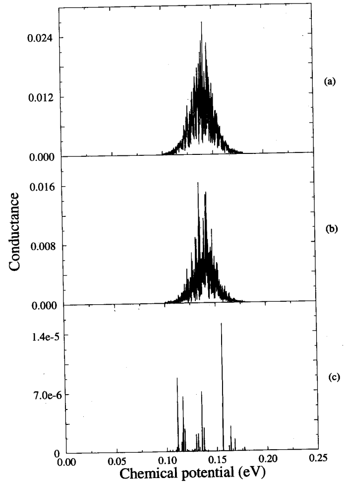
Fig. 4. dc conductance at 77 K as a function of chemical potential for (a) perfect ( W = 0 ) DQWSL, (b) imperfect ( W = 0.05 ) DQWSL, and (c) random ( W = 0 ) QWSL. The SL's parameters are the same as in Fig. 3. Note that the scale in figure (c) is much smaller than in the other two ones.
