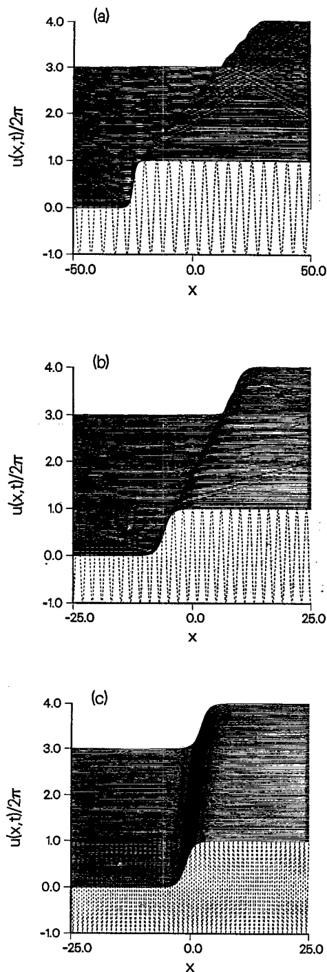
FIG. 1. Absence of radiative divergence for kinks propagating in the spatially periodic SG model. Parameters are (a) k = 2\pi/5 , initial velocity v = v_{\text{thr}} = 0.387726\dots ; (b) k = \pi , initial velocity v = v_{\text{thr}} = 0.091999\dots ; (c) k = 2\pi , initial velocity v = v_{\text{thr}} = 0.024704\dots [corresponding wavelengths are (a) 5, (b) 2, and (c) 1]. In all three cases, \epsilon = 0.4 . The amplitude of the emitted radiation is very small; due to the periodic boundary conditions, it can be seen reentering the simulation interval without any appreciable interaction with the kink. Only half of the simulation interval is shown in plots (b) and (c) to enlarge details. Time increases upwards with final time t = 100 . The potential is indicated by the dashed line (amplitude not to scale).
