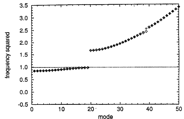
FIG. 10. Spectra for the kink on periodic potentials of wavelengths 5.2 ( \diamond ) and 5.3 ( \times ). Between these two values, the whole first band of the spectrum occurs below the phonon band.
