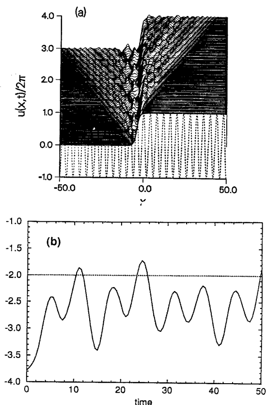
FIG. 6. Trapping of a kink at an intermediate position in the potential instead of at the bottom. \epsilon = 2 and the kink starts with velocity 0.1. The amount of emitted radiation is large due to the fast acceleration of the kink in this large perturbation. (a) Time evolution of the kink; (b) time evolution of the center of mass. The neighboring minimum is at x = -2.0 (indicated by the dashed line) and the kink oscillates around approximately x = -2.5 . The final time is t = 50 .
