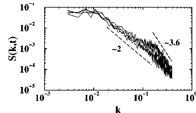
FIG. 15. Power spectrum of an interface with r=0.5, p=0.5, s=1 , and c=0.1 at times 10^7, 2 \times 10^7, 3 \times 10^7, 4 \times 10^7, and 5 \times 10^7 . Power spectra are anomalous at short scales. Dashed lines are guides to the eye.
