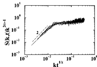
FIG. 13. Collapsed power spectrum with p=2, s=1, r=0.1 , and c=0.05 using the Edwards-Wilkinson universality class exponents at six equally spaced times from 8 \times 10^6 to 3 \times 10^7 . Dashed line has slope 2\alpha + 1 = 2 .
