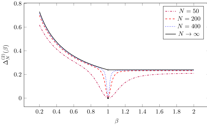
Fig. 6. Values of \Delta_N^{(v)}(\beta) for \nu = 2 and different values of N : the limiting function \lim_{N \rightarrow \infty} \Delta_N^{(2)}(\beta) is also represented, including its discontinuity for \beta = 1 .
