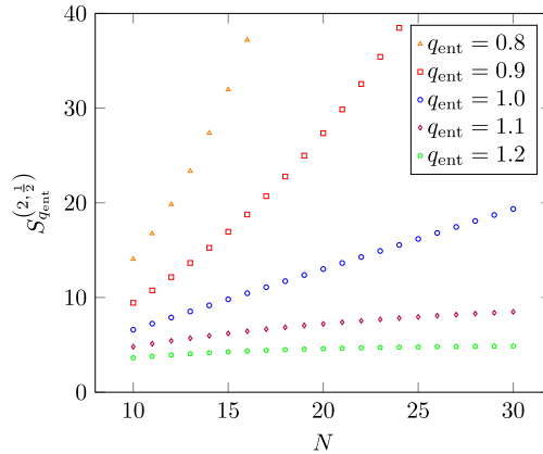
Fig. 2. Values of the S_{q_{ent}}^{(2,\alpha)} entropy (32) for \alpha = \frac{1}{2} versus N for different values of q_{ent} .
