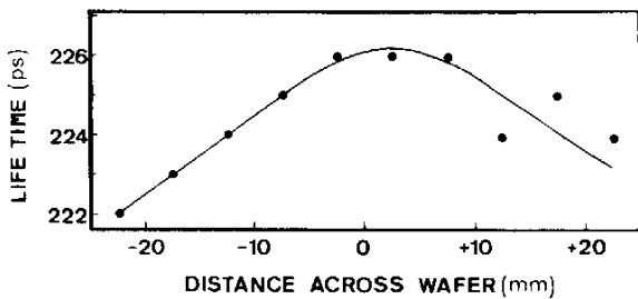
FIG. 6. Positron lifetime across the wafer diameter. The absolute error is 1.5 ps.
