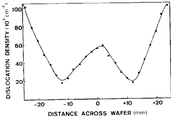
FIG. 2. Dislocation density across the wafer diameter.
